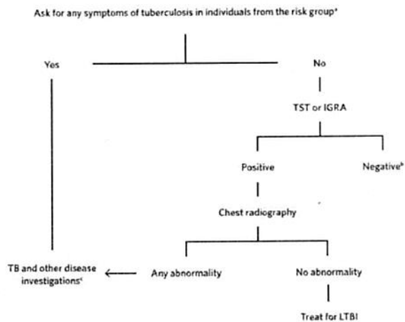
Fig. 4 Algorithm for targeted diagnosis and treatment of LTBI and exclusion of active TB in HIV-negative household contacts aged \geq 5 years and other at-risk populations
